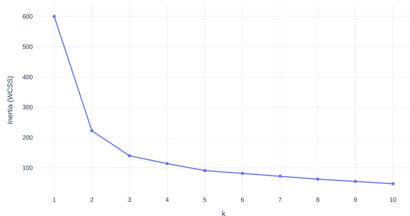
Fig. 2.3: Plotly elbow chart
